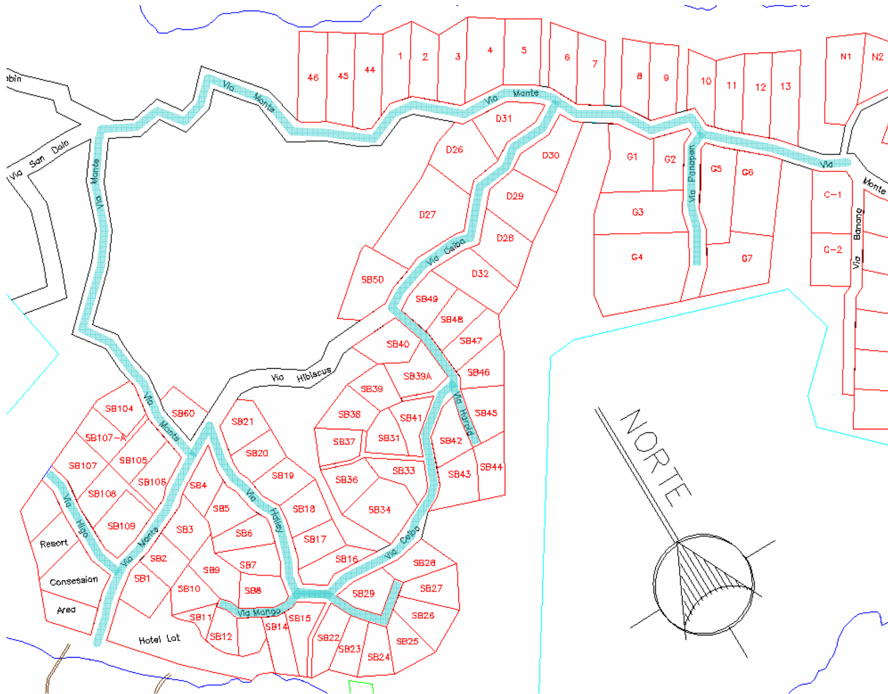
Cart Paths highlighted in blue have been Rough Graded; cut and fill, and Culvert bridges installed for accessibility of Golf Carts. These also indicate the areas ready for the Underground Utilities and stub ups to each lot corner prior to the finish grade, surfacing and landscaping.
